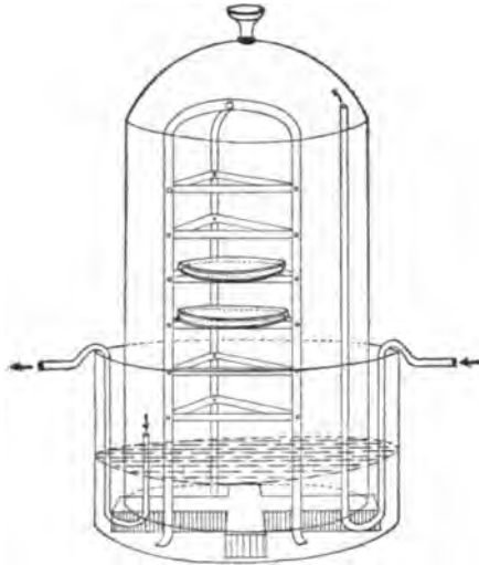
FIG. 134.—Botkin's apparatus.
